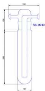
Type SL 29-KZ
