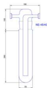
Type SL 29-NW16-Z / NW25-Z
