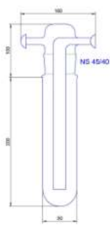
Type S 29-KZ
