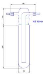
Type S 29-GL-Z
