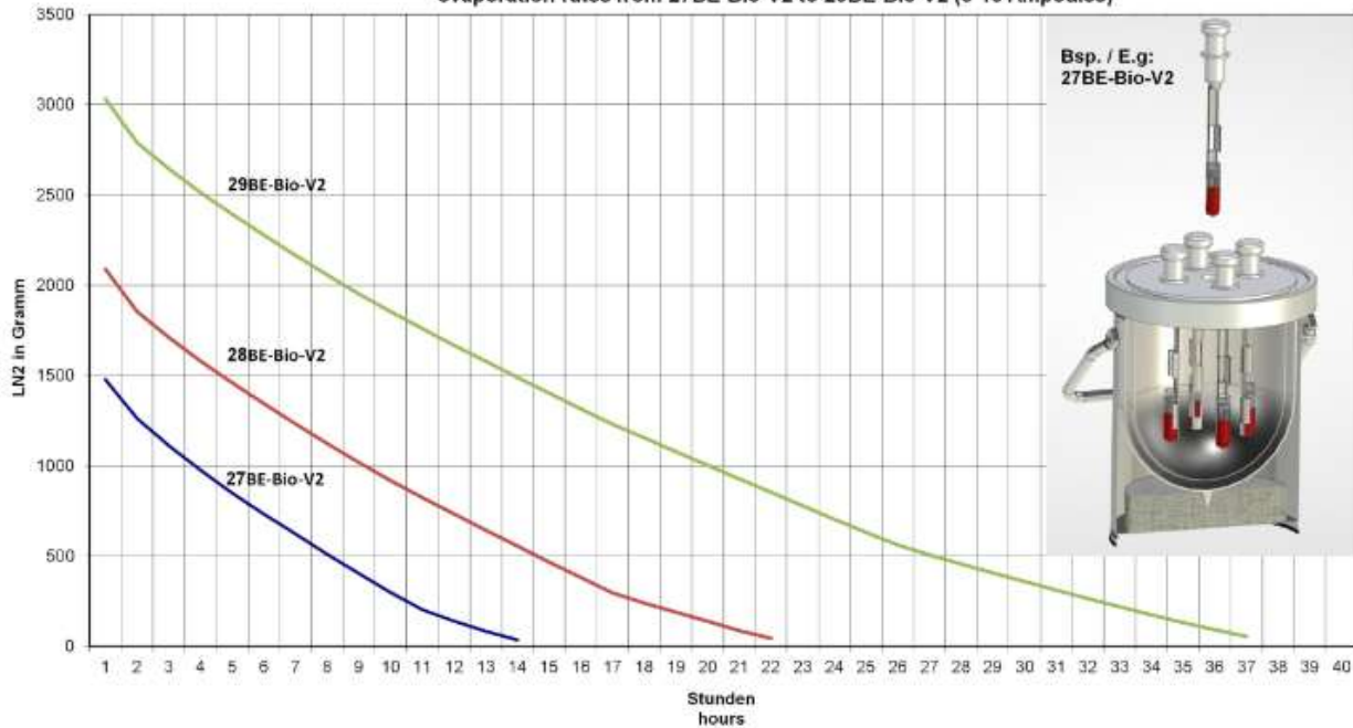
Verdampfungsraten von 27BE-Bio-V2 bis 29BE-Bio-V2 (5 -15 Ampullen) evaporation rates from 27BE-Bio-V2 to 29BE-Bio-V2 (5-15 Ampoules)
